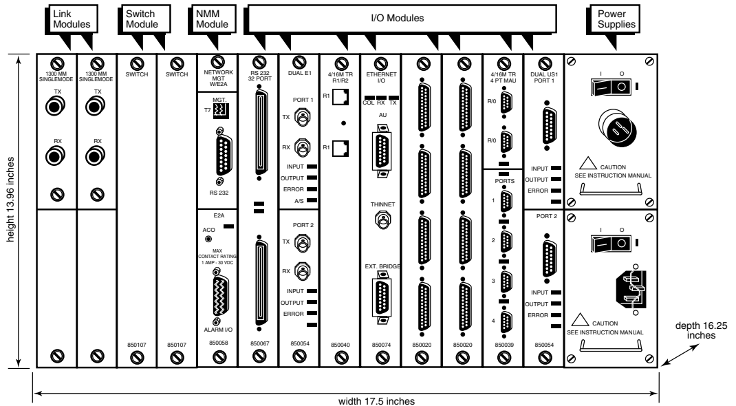
Figure 1. PremNet 5000 Chassis
