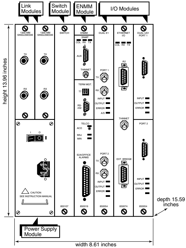
Figure 2. PremNet Branch Chassis
